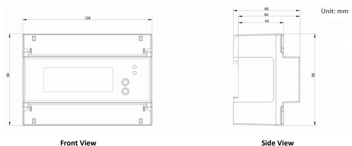
Figure 2-2 Dimensions
