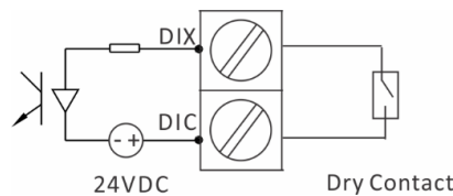
Figure 2-8 DI Connections
