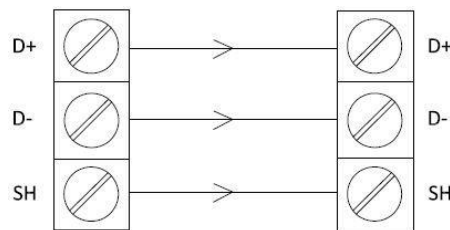
Figure 2-7 RS-485 Connections
