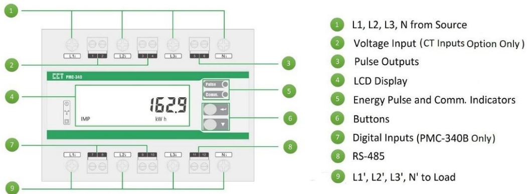
Figure 2-1 Appearance
