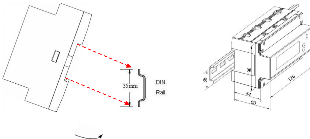
Figure 2-4 Installation
