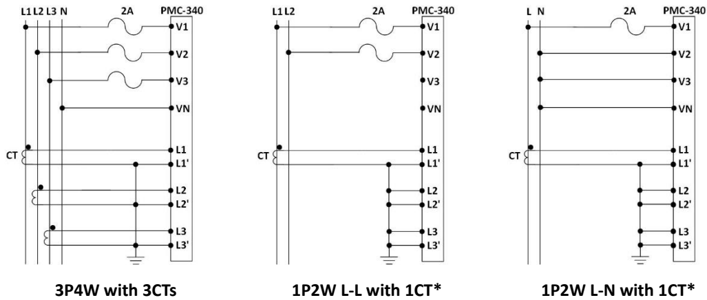
Figure 2-6 CT Input connections
